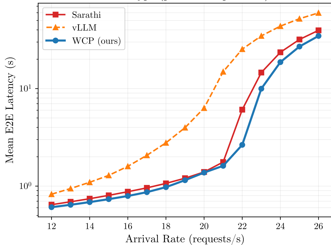
Multi-type (p512d20 + p512d50)
