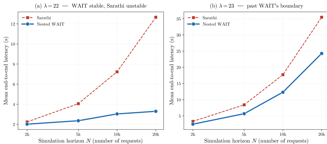
Figure 10 Long-horizon validation on the two-type workload (0.7p512d20, 0.3p512d50). (a) At \lambda = 22 , Nested WAIT approaches a finite latency plateau, whereas Sarathi's mean latency grows roughly linearly in N . (b) At \lambda = 23 , both policies are unstable, but Nested WAIT remains substantially below Sarathi at every horizon we consider.
