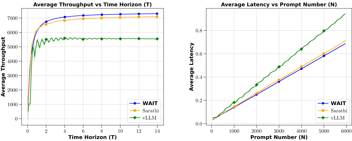
FIGURE 7. Average throughput and latency across algorithms on the synthetic dataset with low demand.
