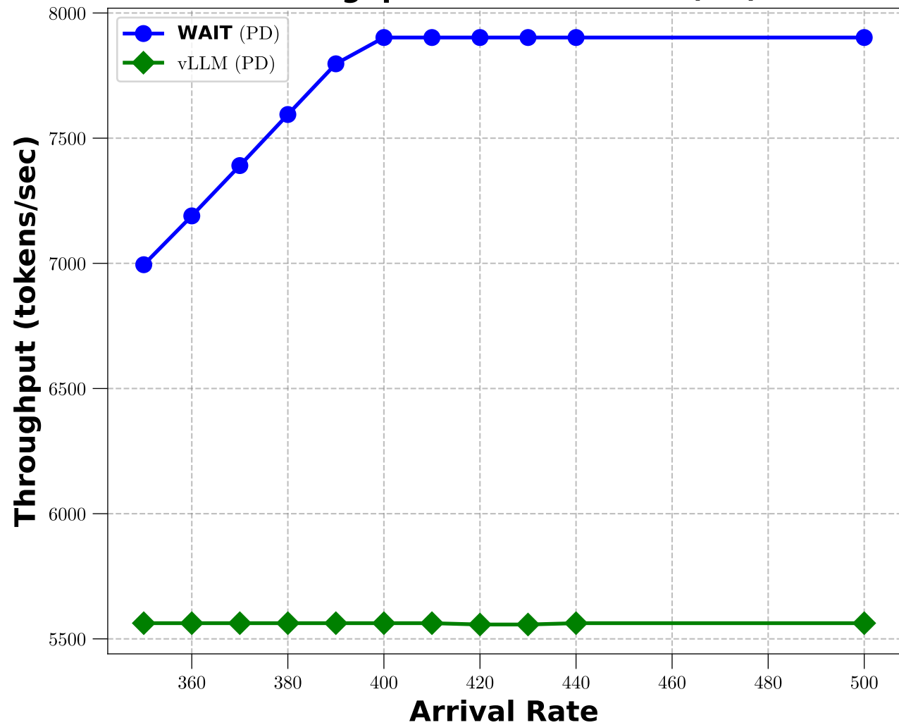
Throughput vs Arrival Rate (PD)
