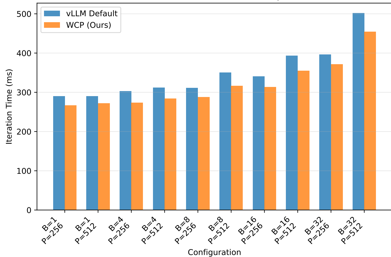
WCP vs vLLM: Iteration Time Comparison
