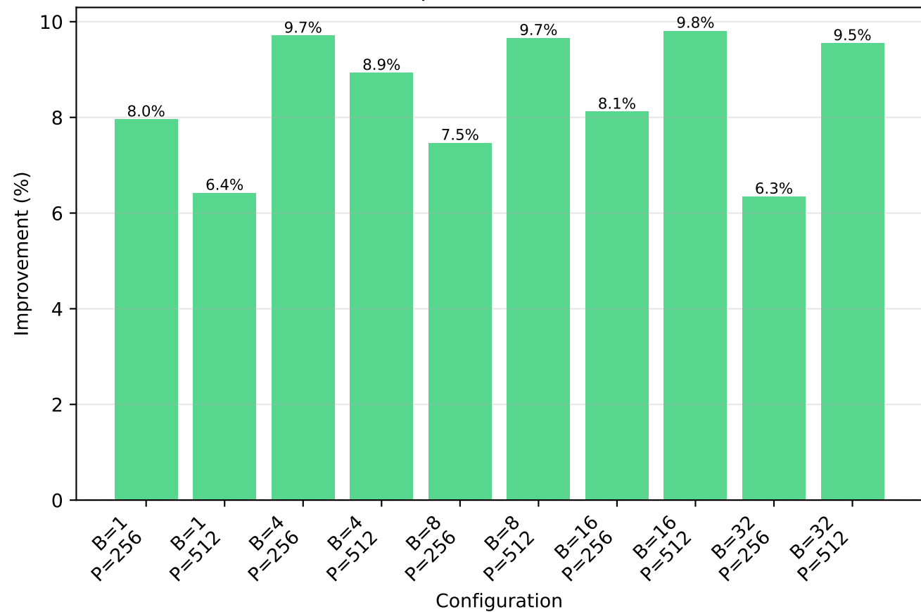
WCP Improvement over vLLM
