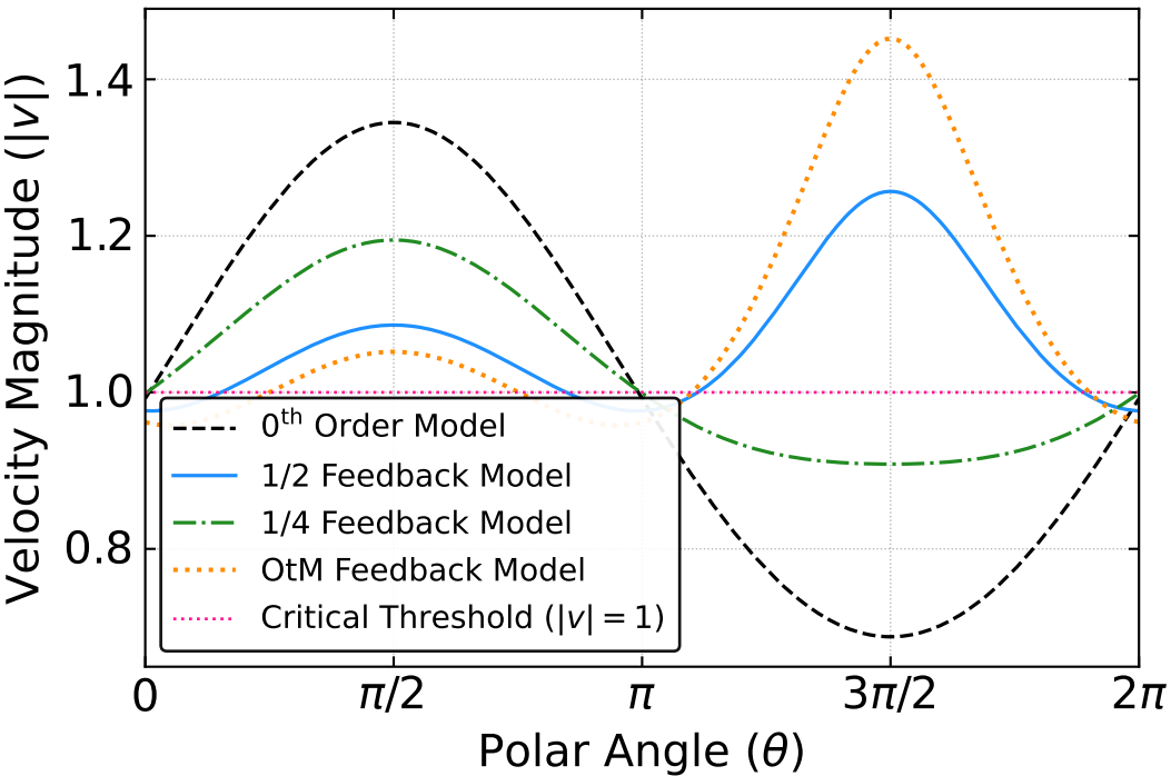
Boundary Surface Velocity Comparison ( c = 0.1 )
