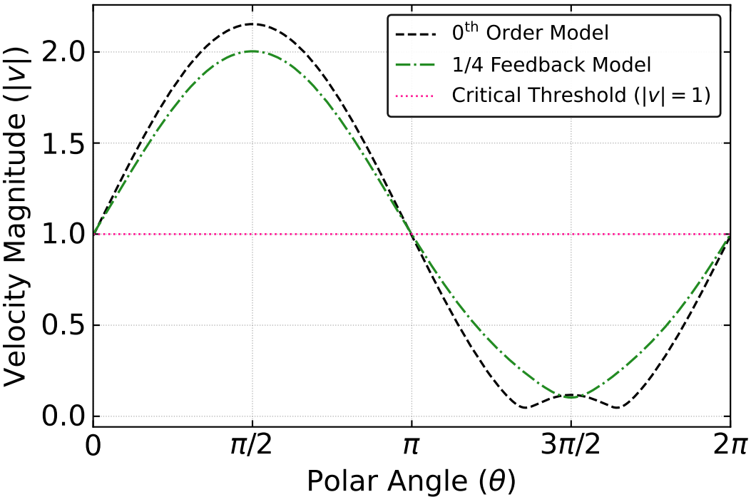
Boundary Surface Velocity Comparison ( c = 0.5 )
