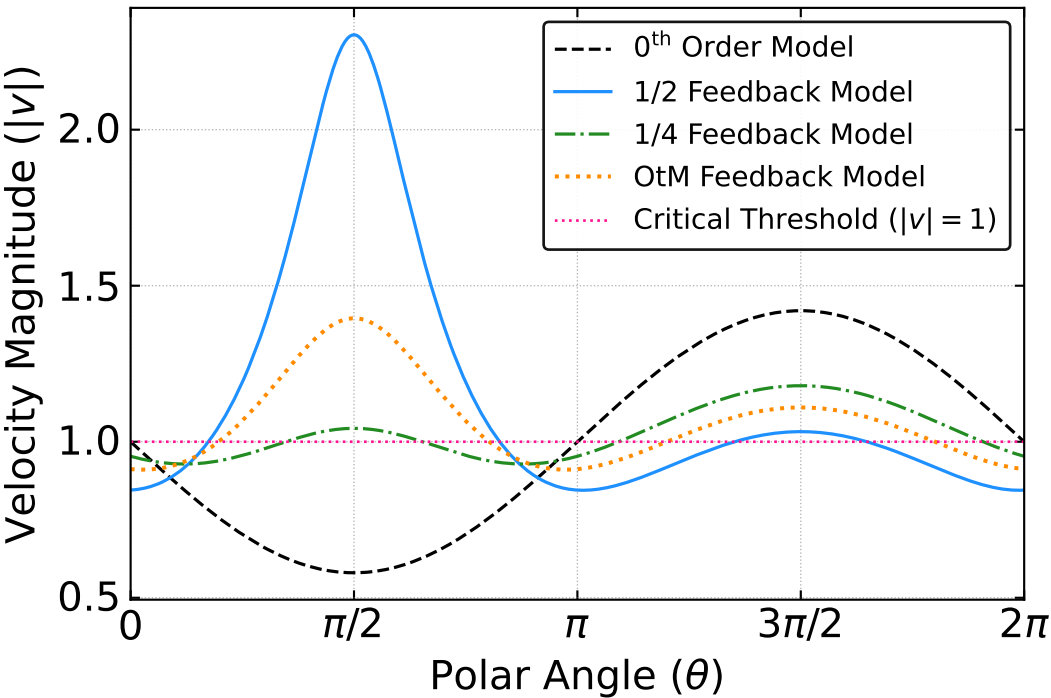
Boundary Surface Velocity Comparison ( j_0 = 0.21 )
