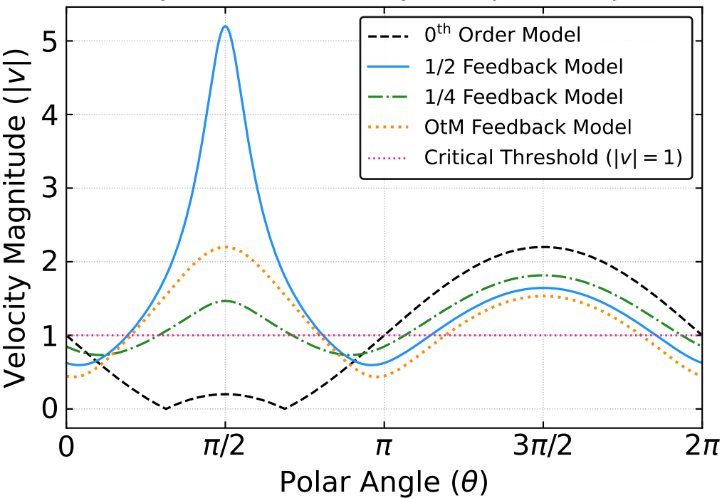
Boundary Surface Velocity Comparison ( j_0 = 0.6 )
