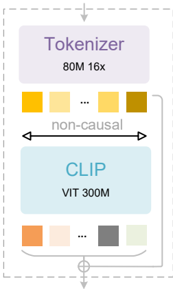
DeepEncoder
