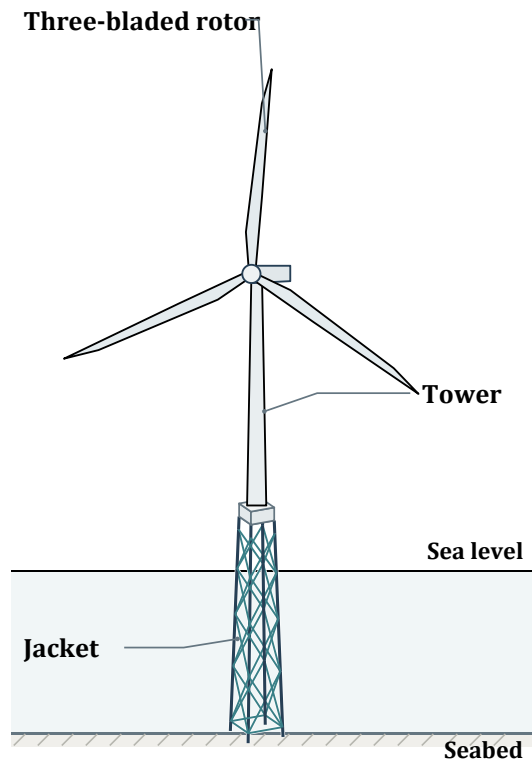
Bottom-fixed four-legged jacket
