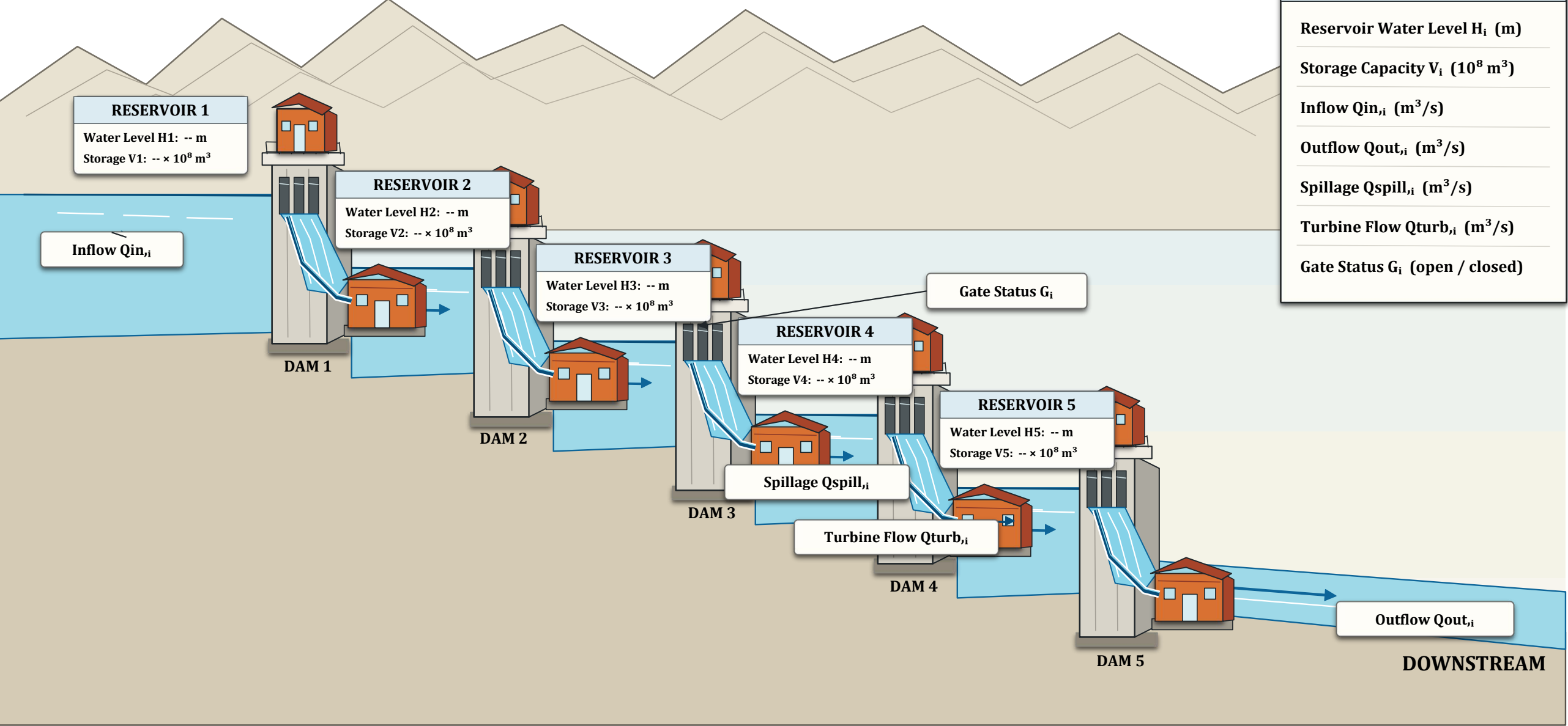
(b) Cascade reservoir operational data schematic
