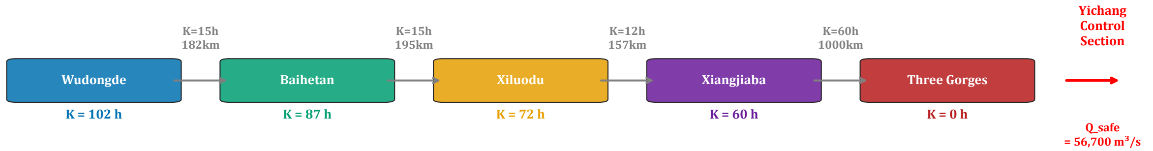
(a) Cascade topology and Muskingum routing lags
