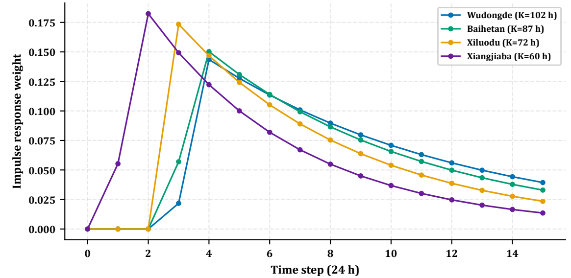
(c) Muskingum impulse response to control section
