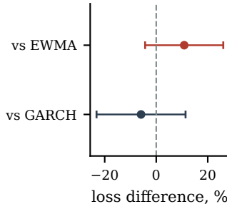
minimum variance
