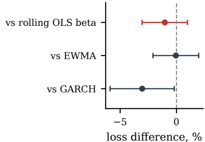
hedging
