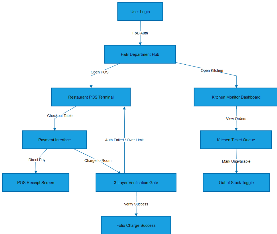
Figure 4: F&B Screen Flow
