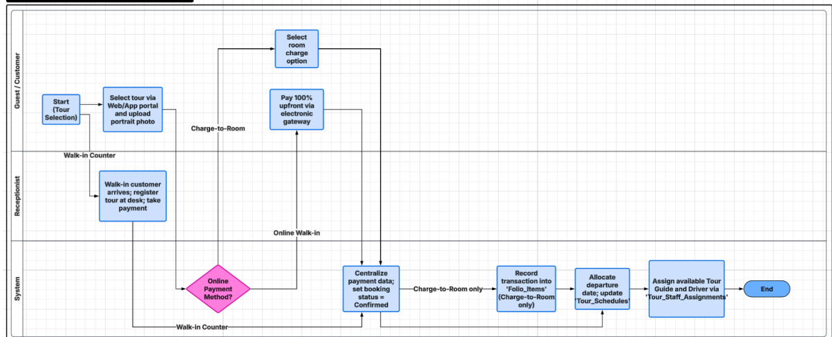
Tour Booking & Staff Allocation Workflow (Kawal Resort)
