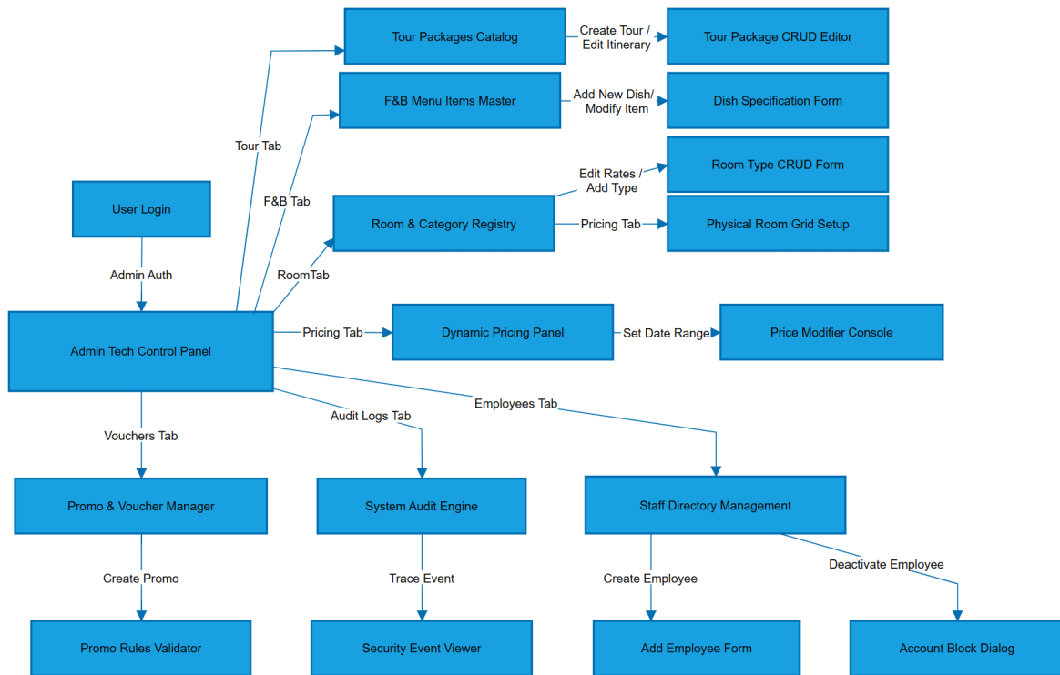
Figure 6: Admin Screen Flow
