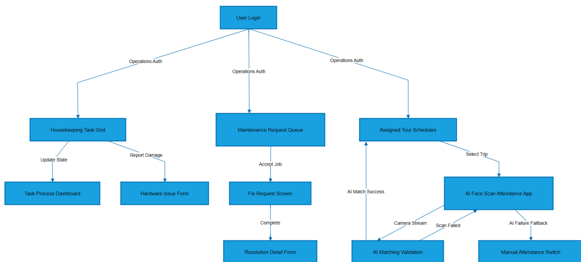
Figure 2: Housekeeping&Maintainer Screen Flow
