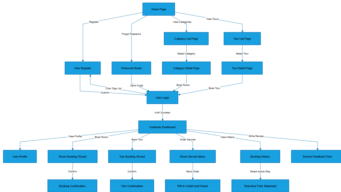
Figure 1: UserScreen Screen Flow
