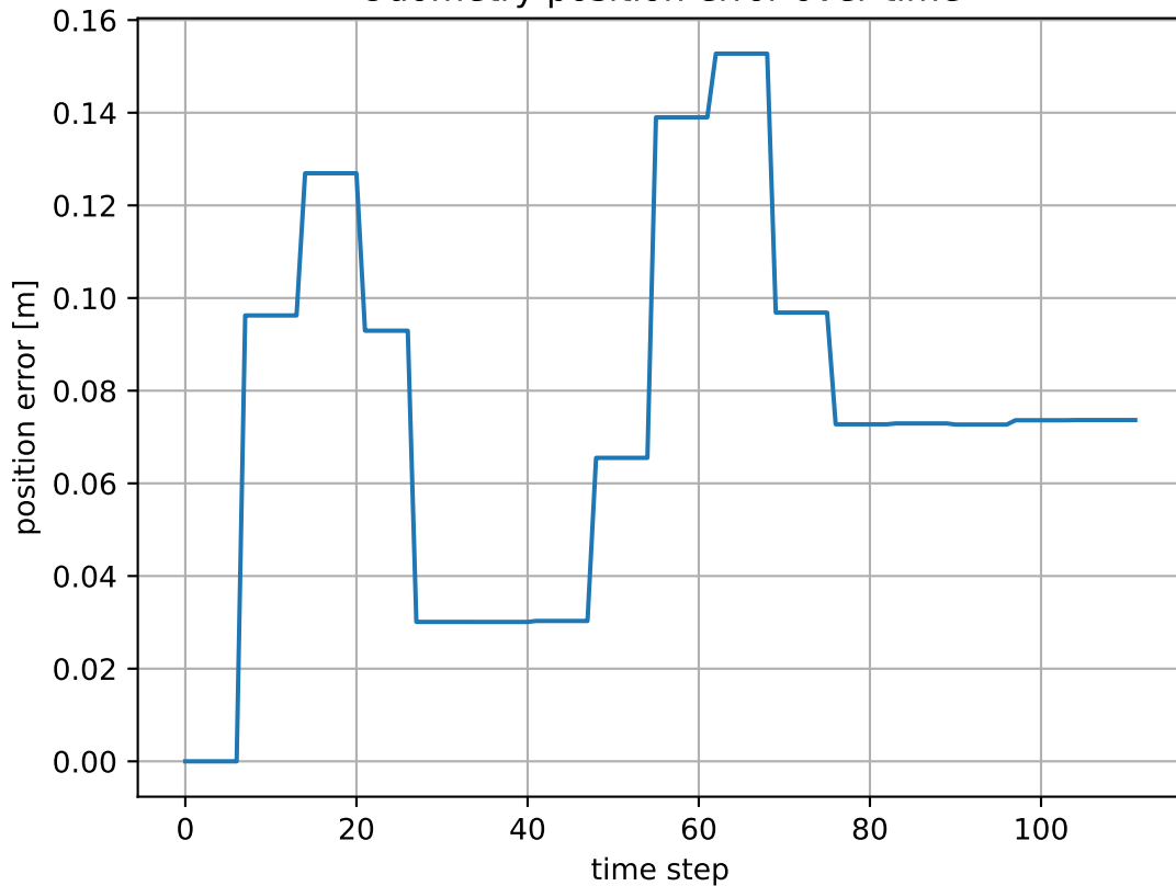
Odometry position error over time
