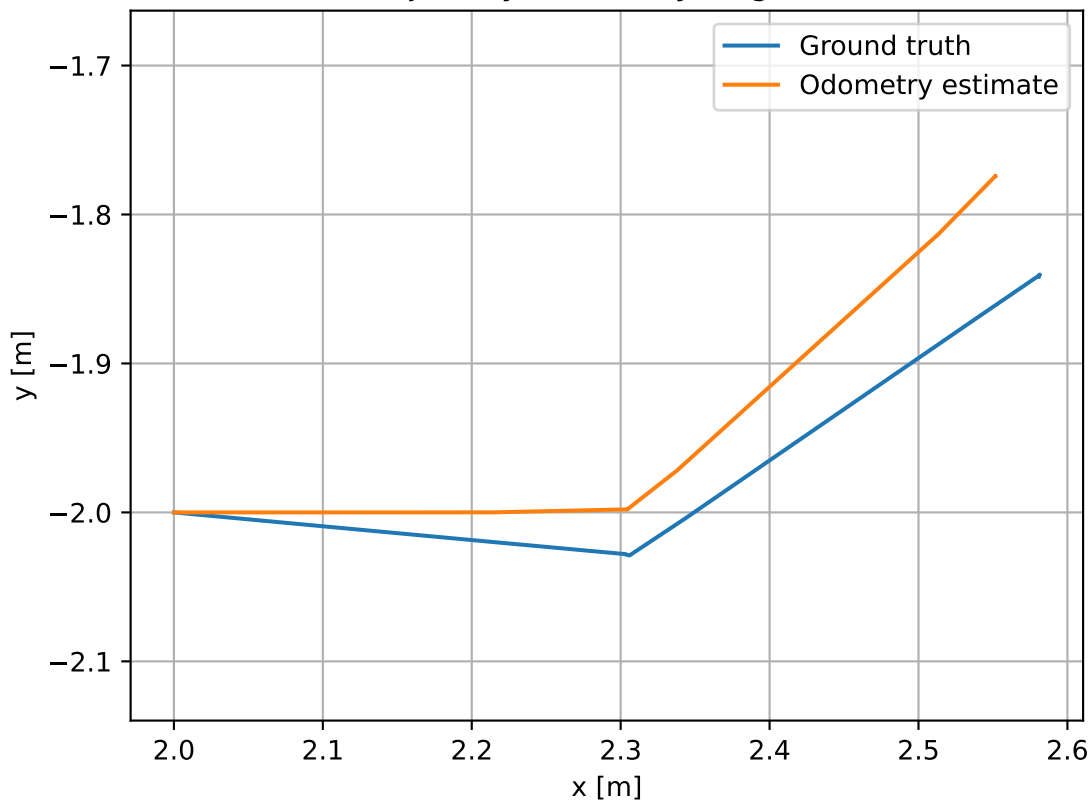
Robot trajectory: odometry vs ground truth
