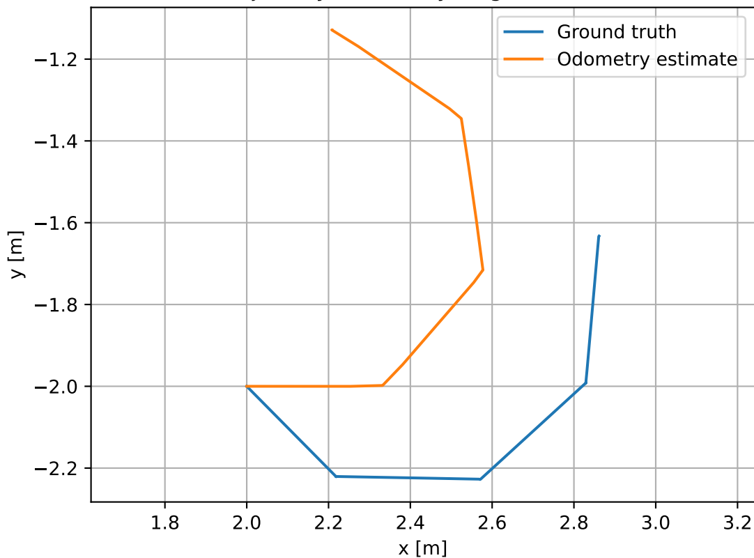
Robot trajectory: odometry vs ground truth (bad)
