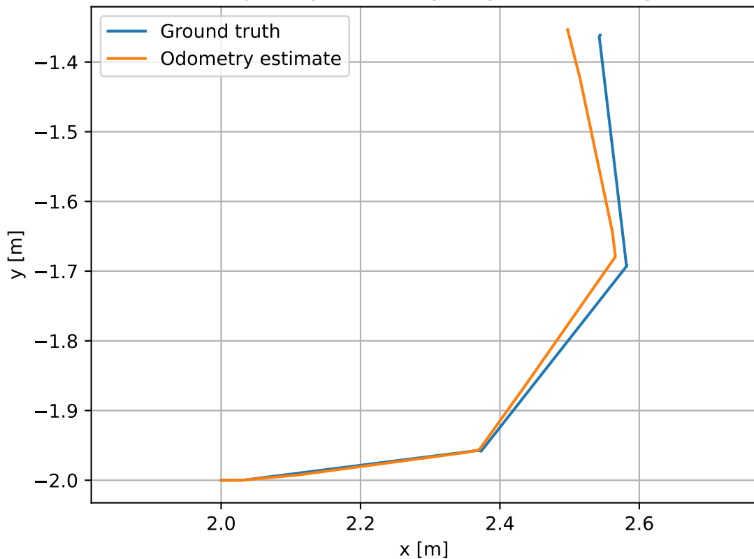
Robot trajectory: odometry vs ground truth (good)
