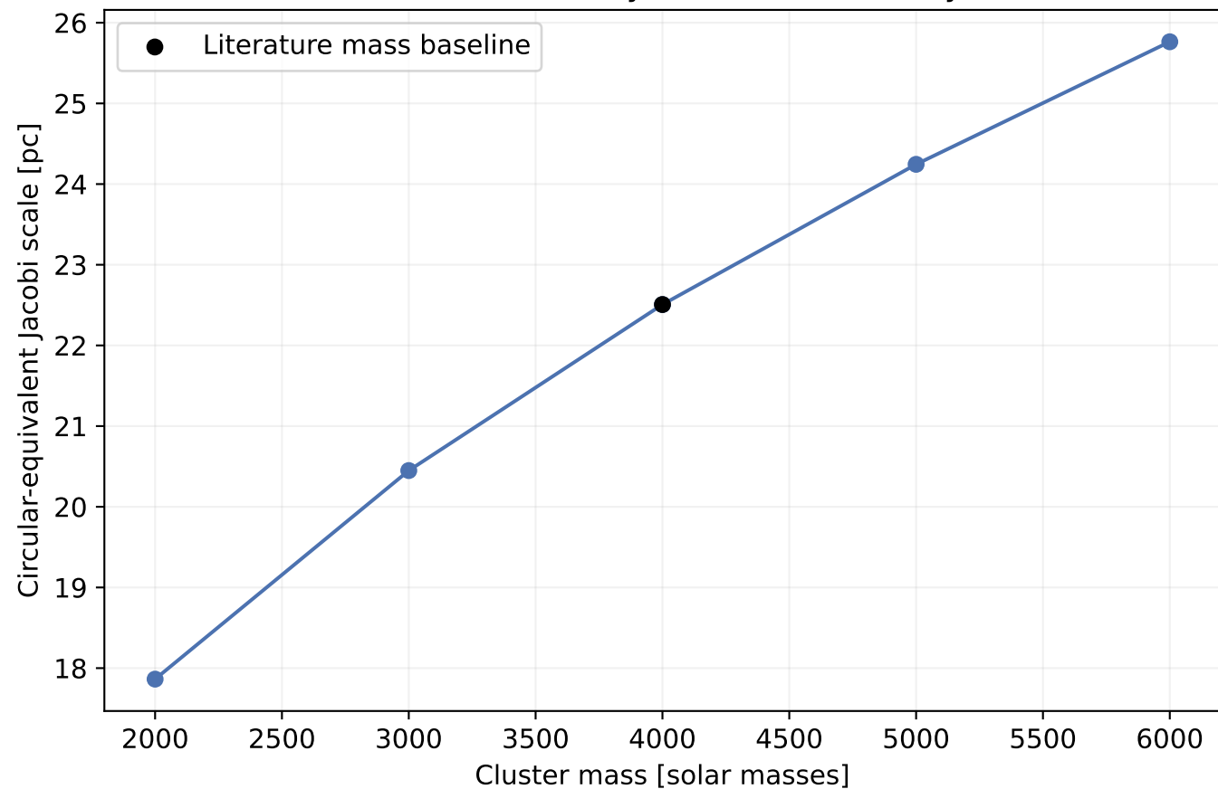
Stock 2 — mass sensitivity (not an uncertainty interval)
