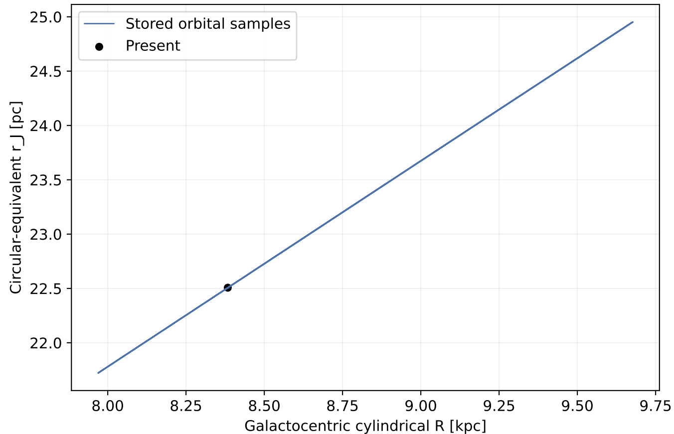
Stock 2 — radial variation of the tidal scale
