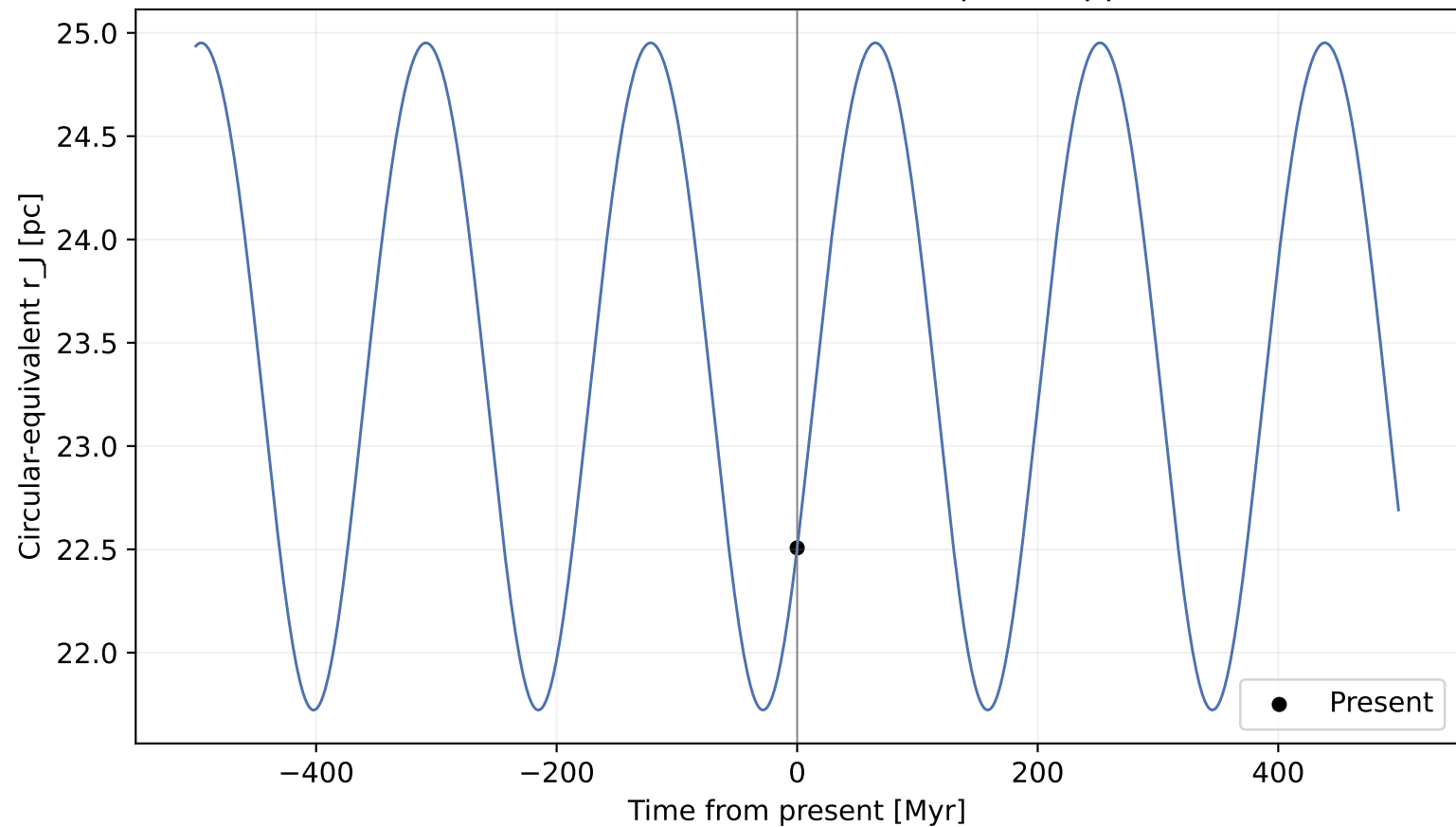
Stock 2 — fixed 4000 solar masses, midplane approximation
