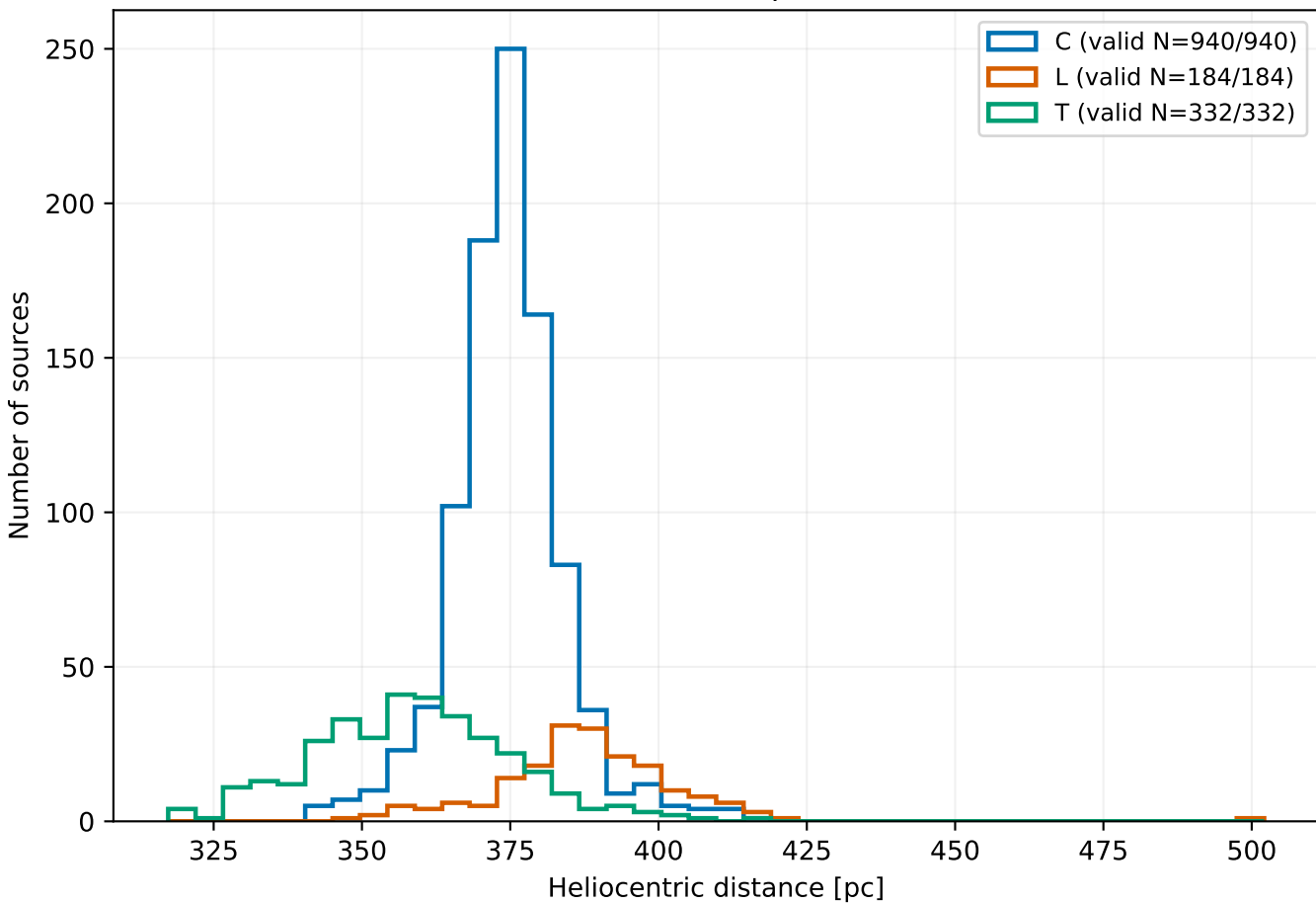
Stock 2 — direct inverse-parallax distances
