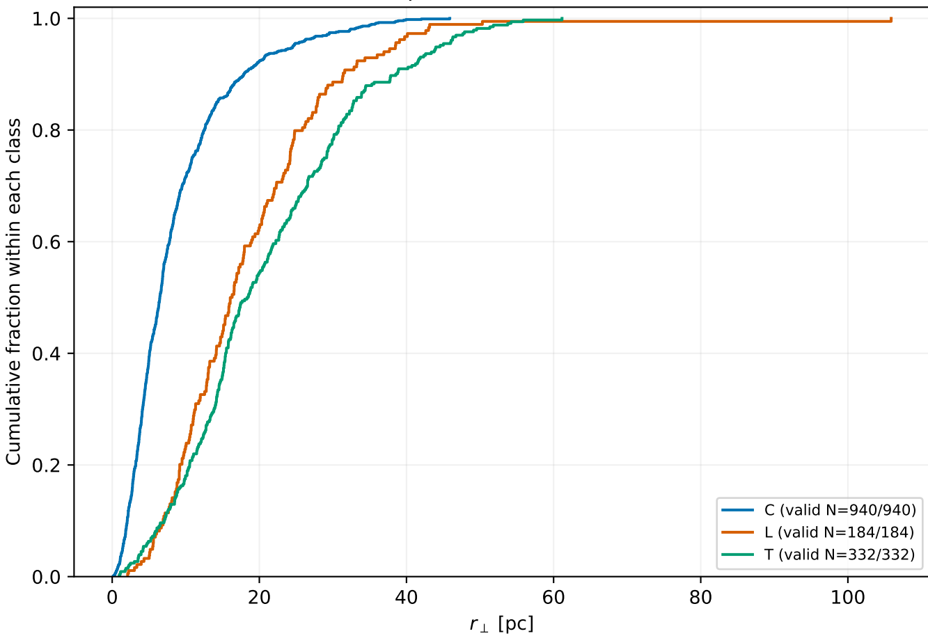
Stock 2 — empirical cumulative distributions
