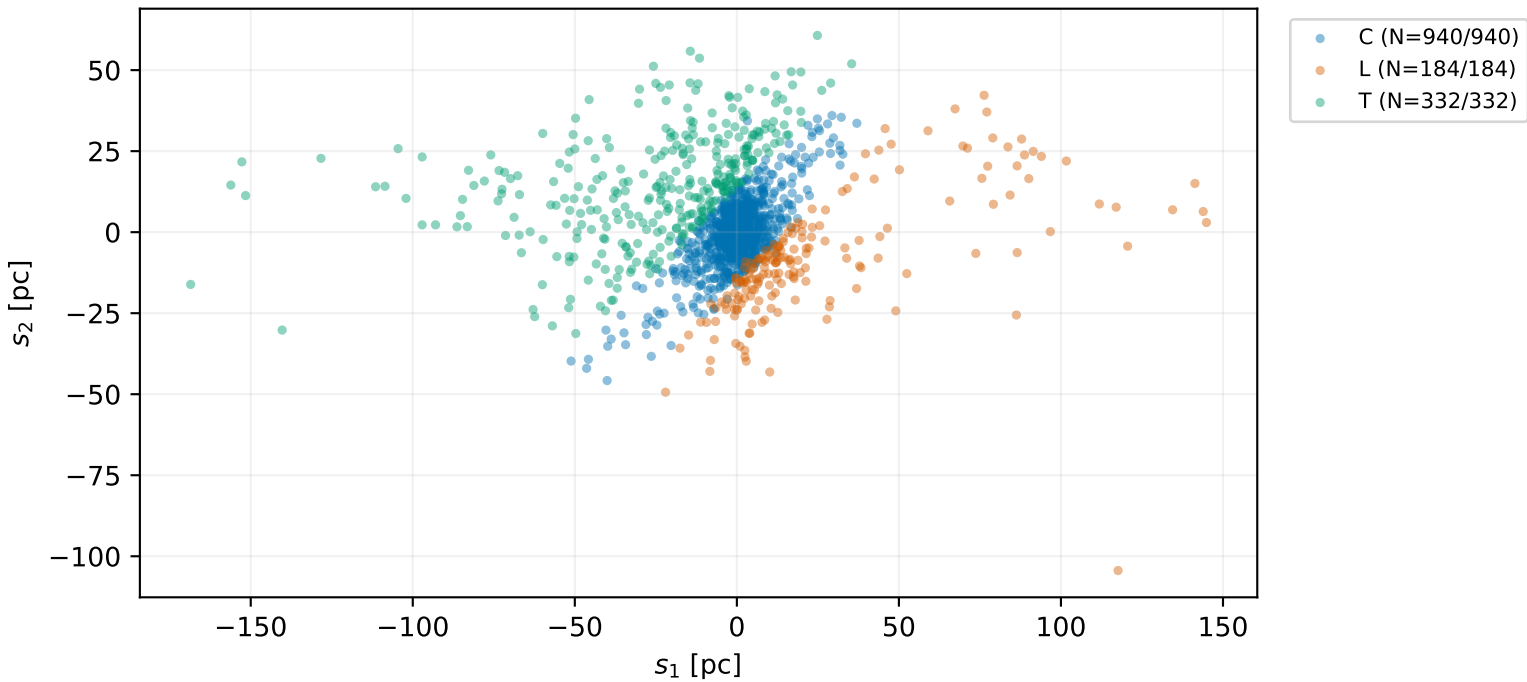
Stock 2 — fixed literature L+T spatial PCA basis
