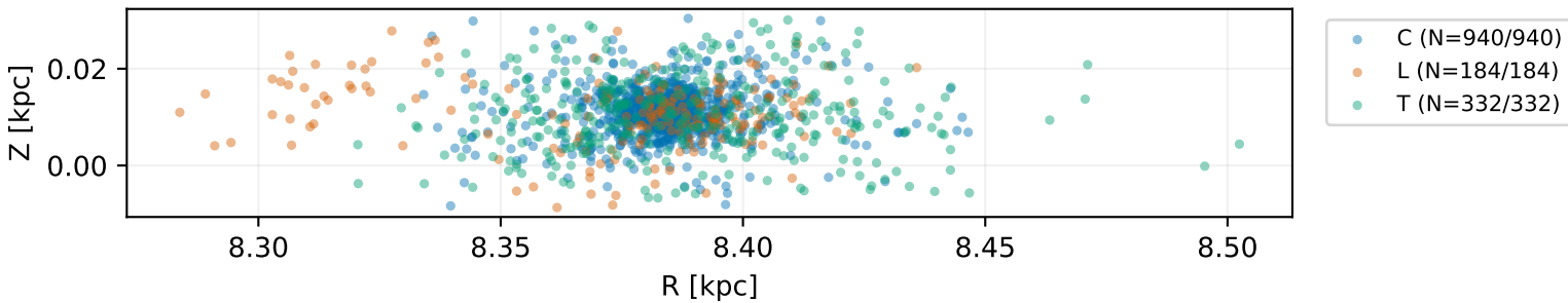
Stock 2 — explicit Galactocentric frame
