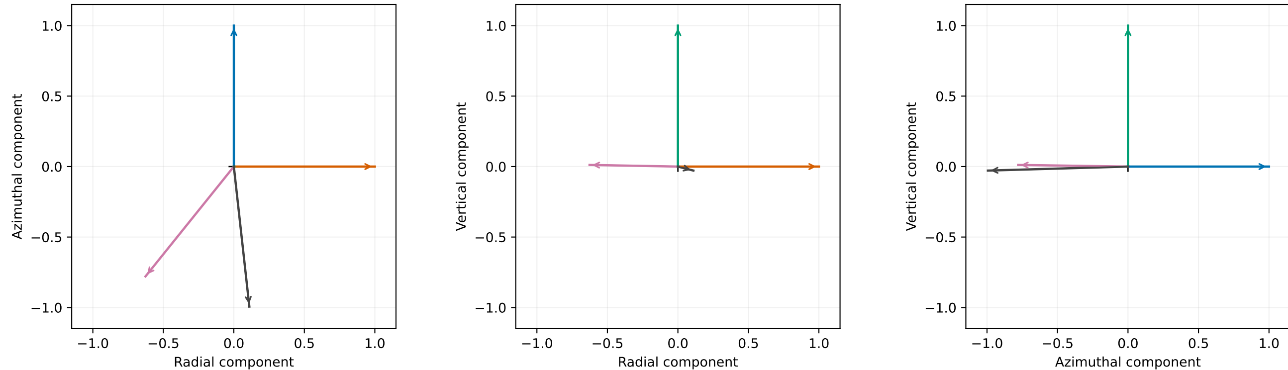
Stock 2 local unit-vector context — direction only; no orbit integrated
