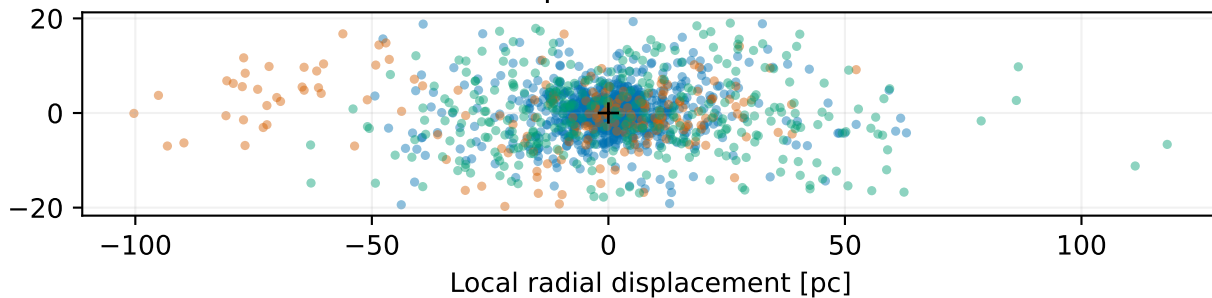
Stock 2 — explicit Galactocentric frame
