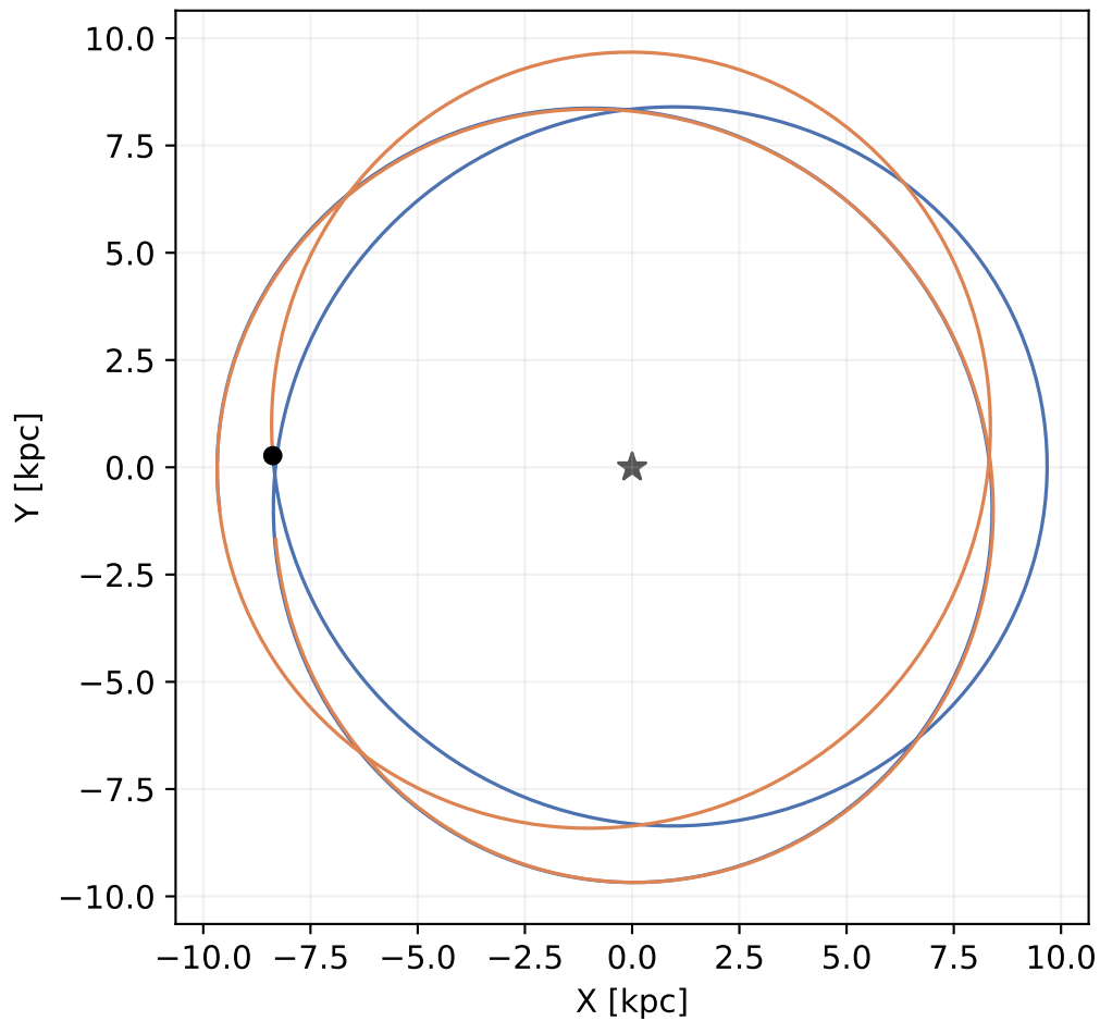
Stock 2 cluster reference orbit
