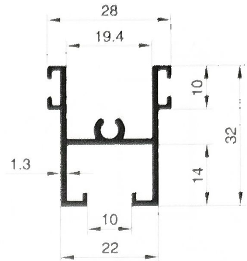
SECTION NO. - 70S-1401 EST. WEIGHT - 0.428 KG./M.
