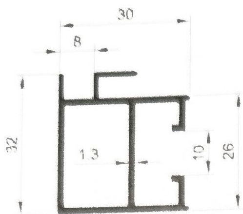
SECTION NO. - 70S-1601 EST. WEIGHT - 0.490 KG./M.
