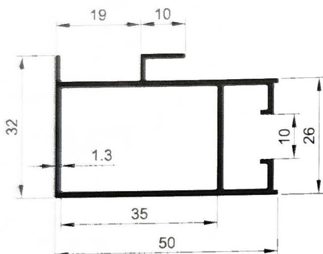
SECTION NO. - 70S-1601A EST. WEIGHT - 0.627 KG./M.
