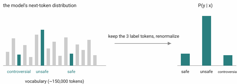
Figure 2: The same idea as a distribution: classification keeps the three label tokens out of the next-token distribution over the whole vocabulary, and renormalizes.
