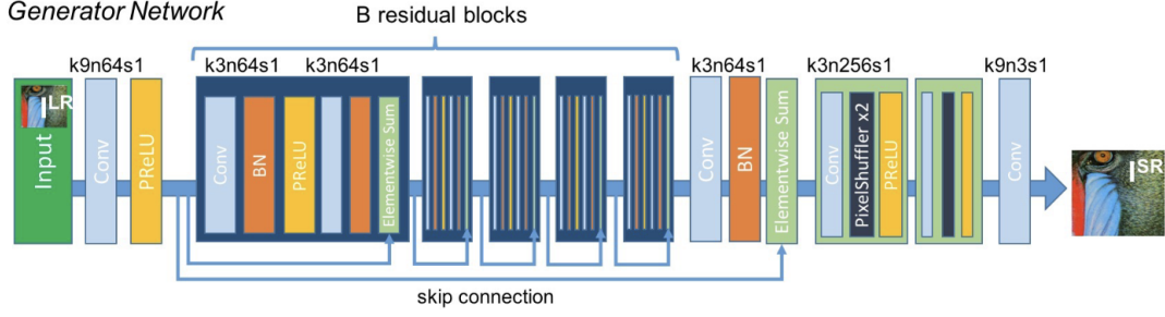
Fig. 3.2. SRResNet generator, after Ledig et al. [33].
