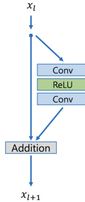
Fig. 3.4. EDSR residual block, after Lim et al. [34].
