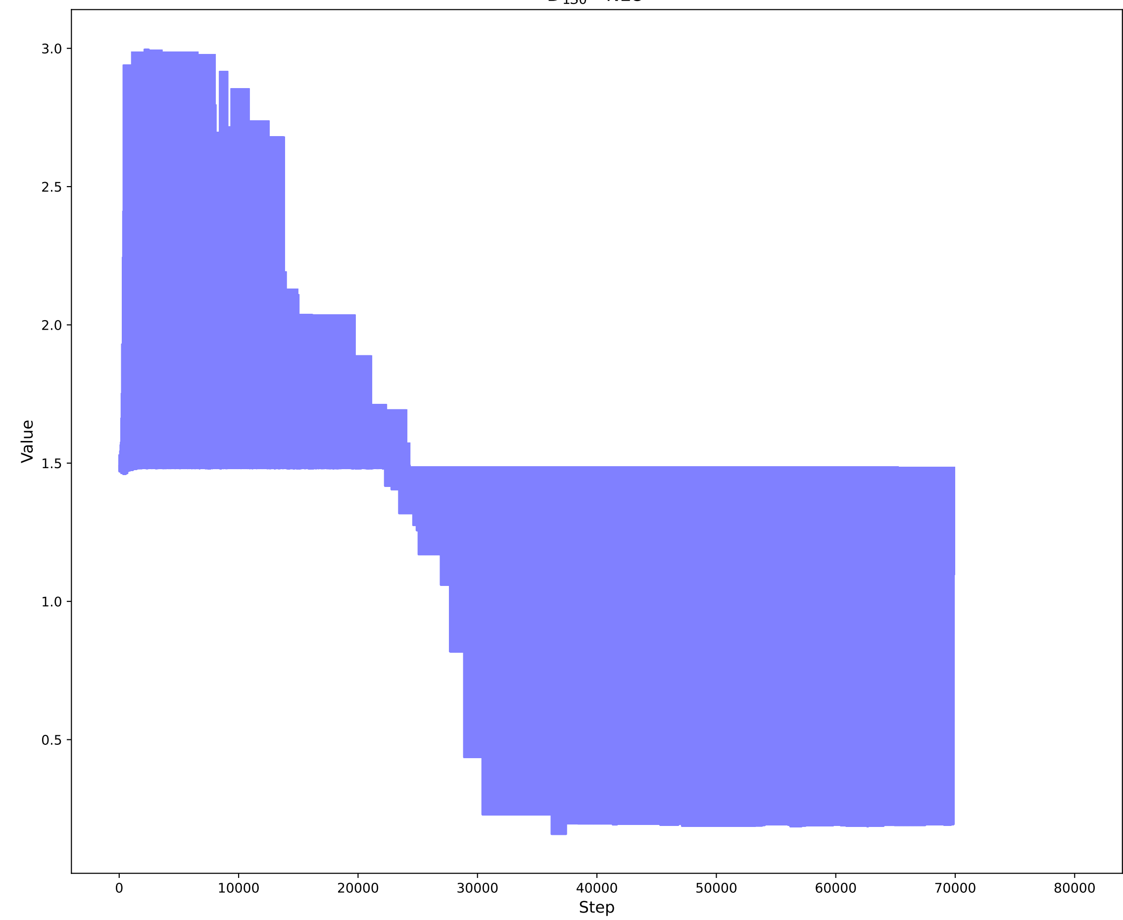
D_{150} - NLO
