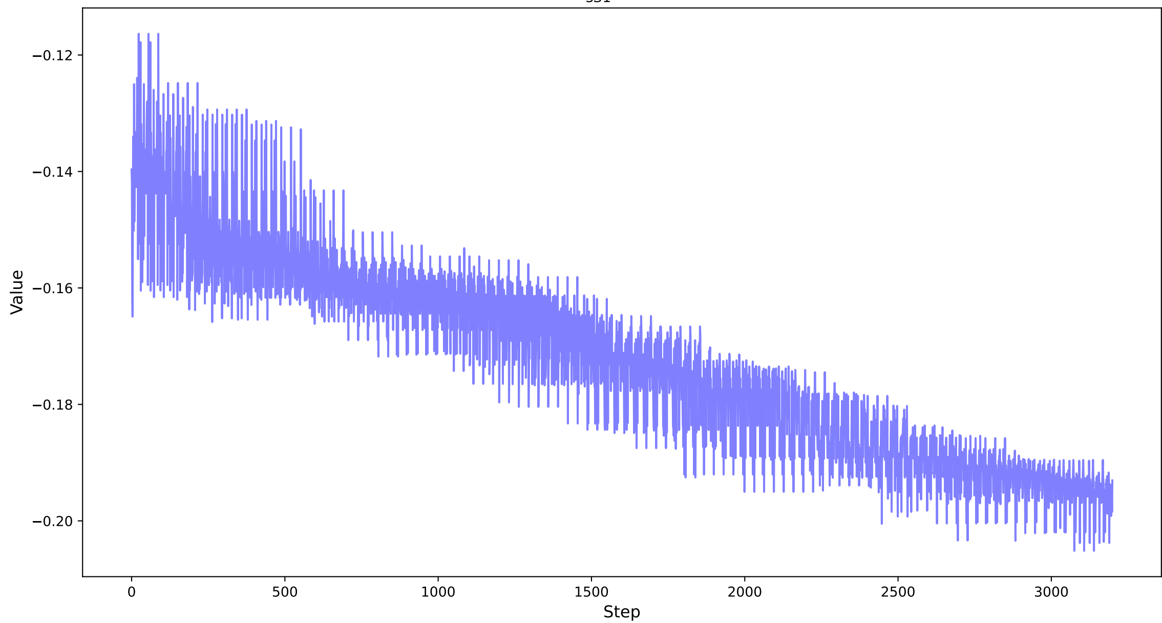
D_{3S1} - NLO
