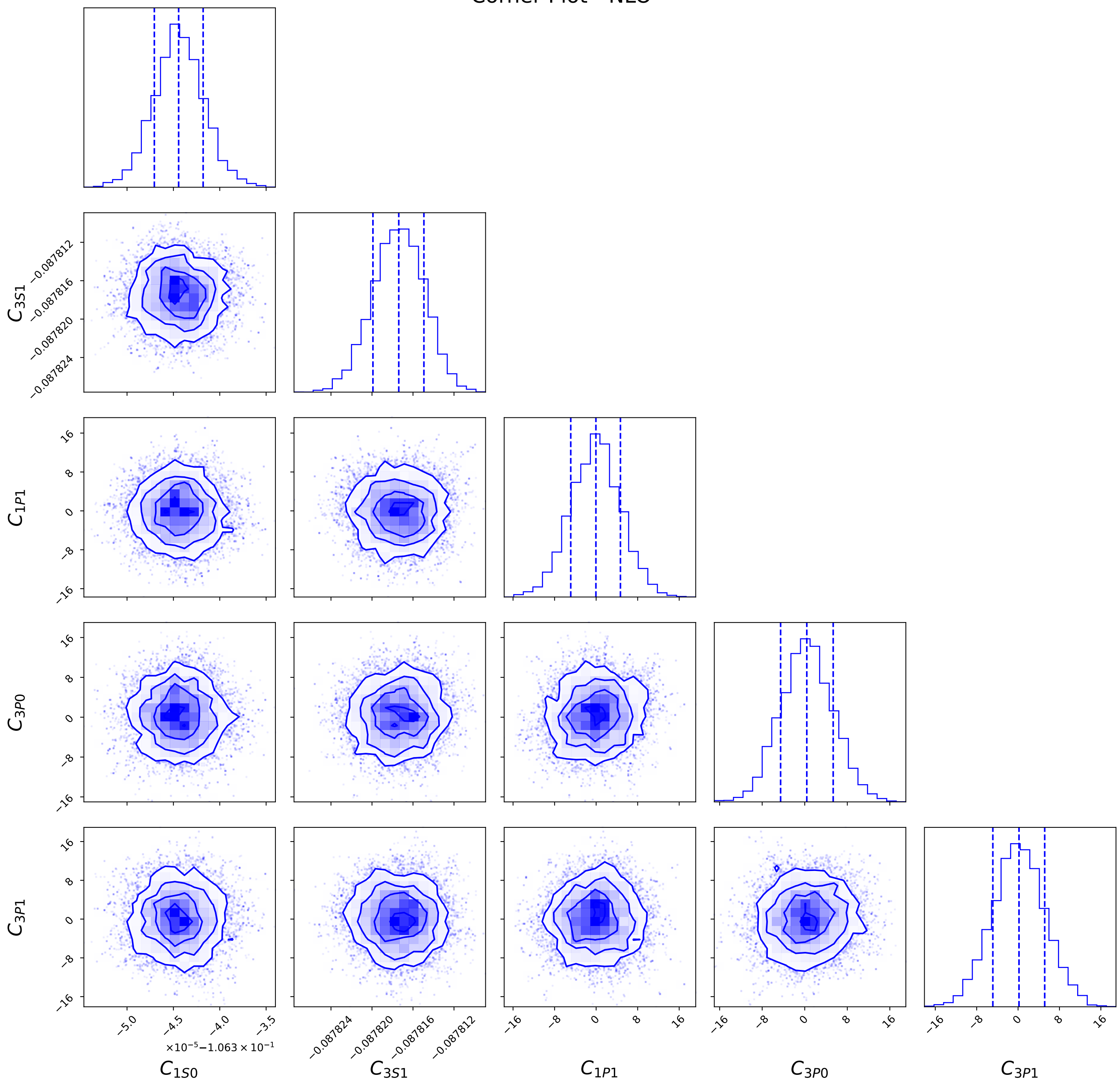
Corner Plot - NLO
