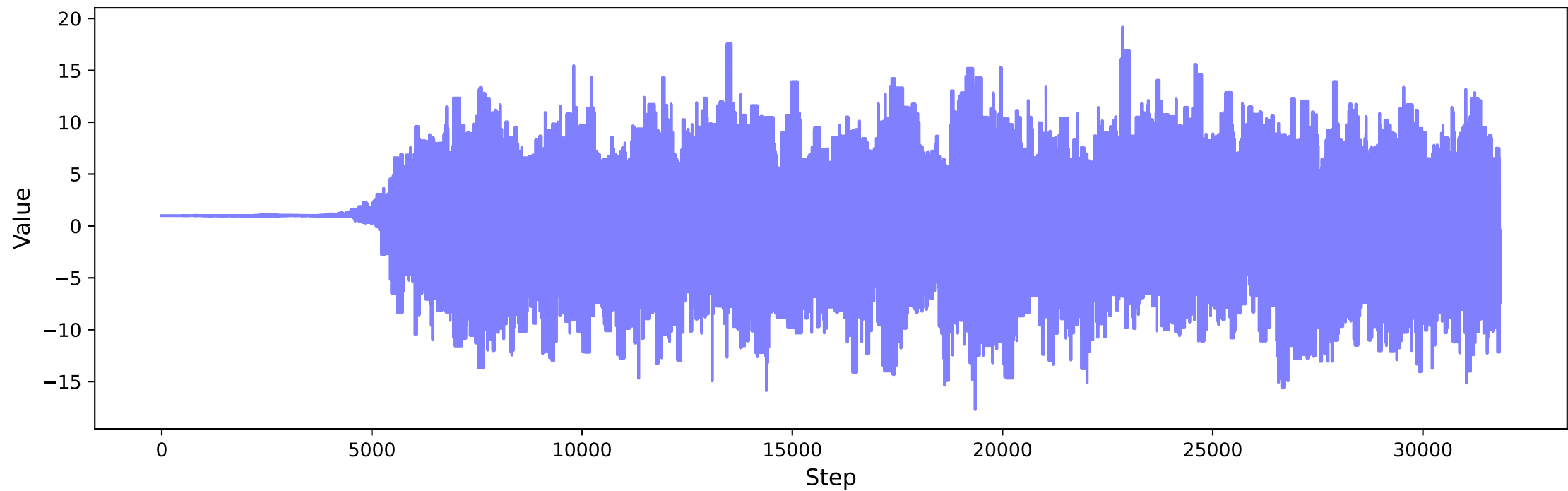
C_{3P0} - NLO
