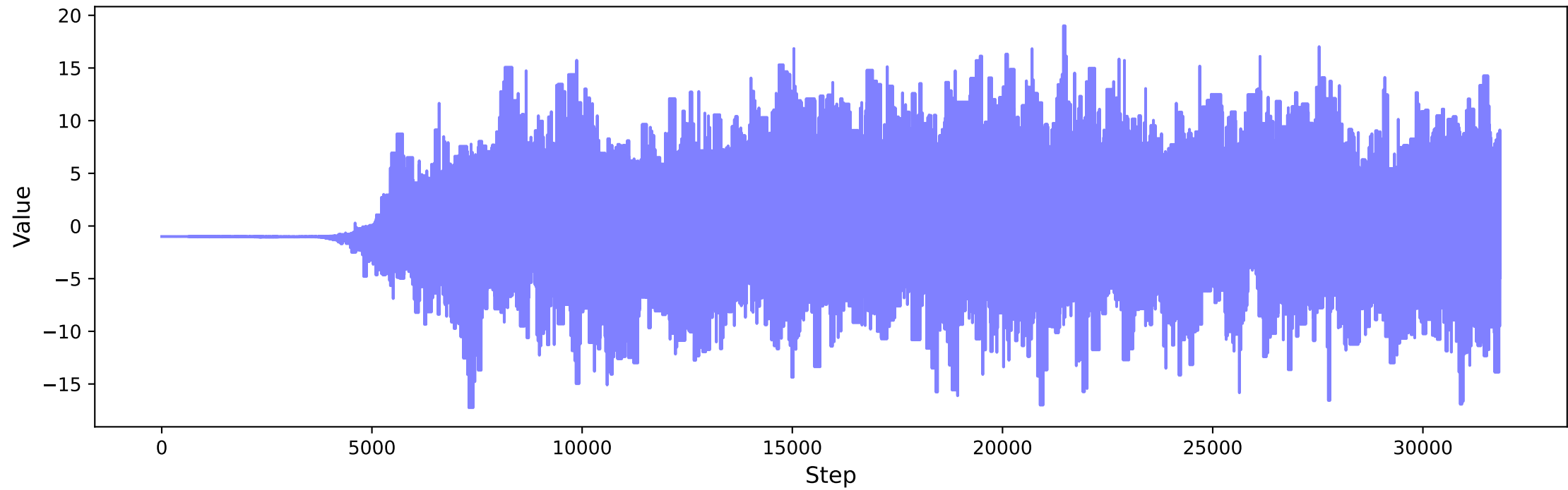
C_{3P1} - NLO
