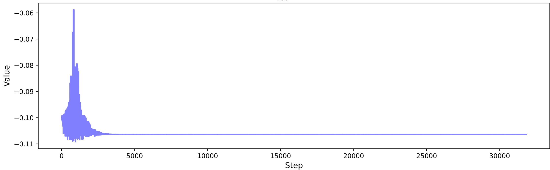
C_{351} - NLO
