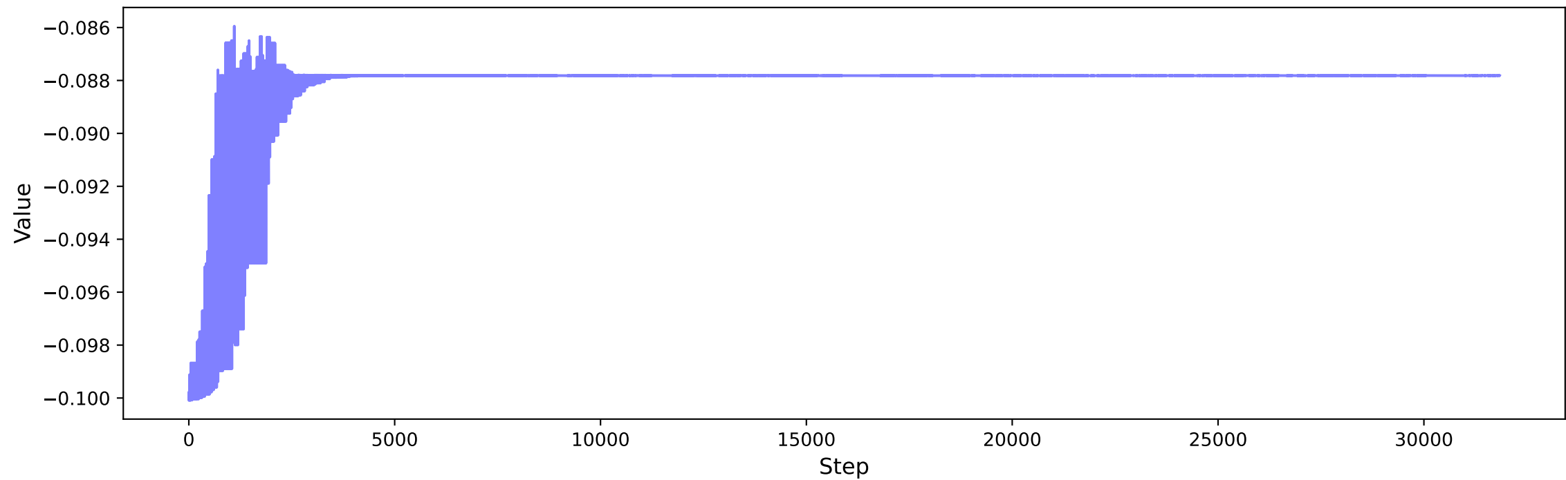
D_{150} - NLO
