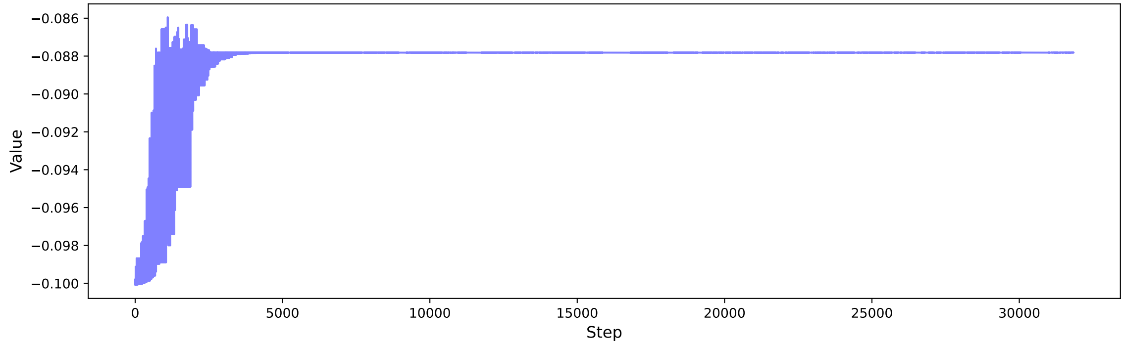
C_{1P1} - NLO
