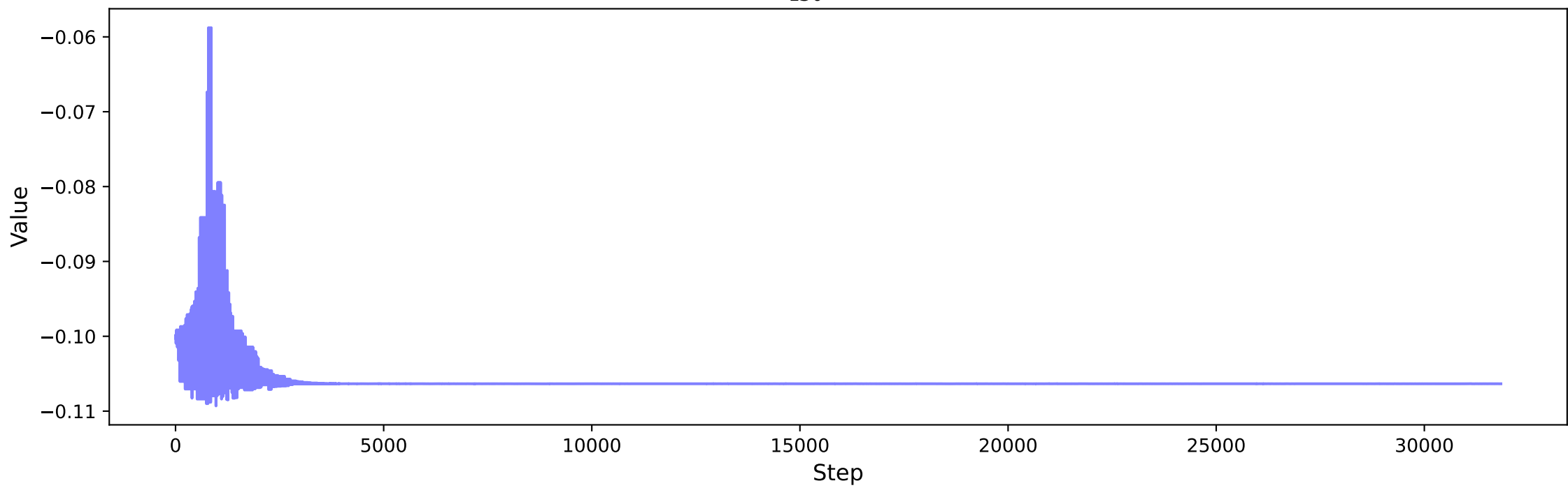
C_{351} - NLO
