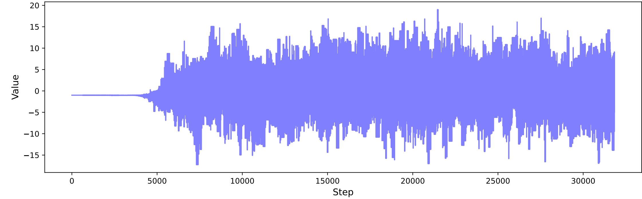
C_{3P1} - NLO
