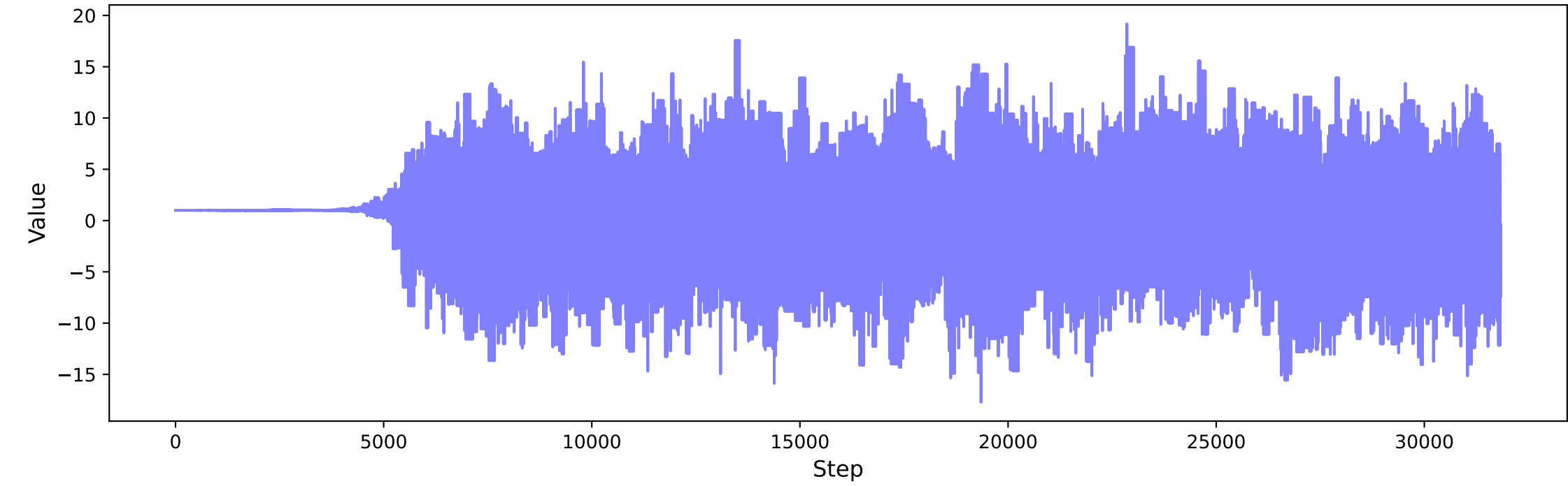
C_{3P0} - NLO
