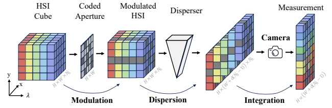
Figure 1: CASSI forward imaging. A spectral cube X is modulated by the coded aperture M , dispersed into shifted spectral measurements, and compressed into a single measurement Y = \Phi X .
