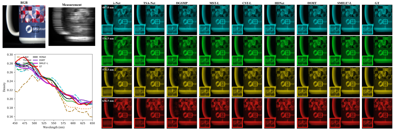
Figure 5: Simulation Scene 5. The figure compares red-green-blue (RGB) reference and measurement inputs, representative spectral bands, zoomed local regions, and spectral density curves.
