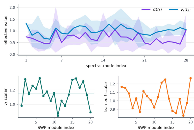
Figure 11: Learned spectral-mode parameters in SMILE 2 -M.
