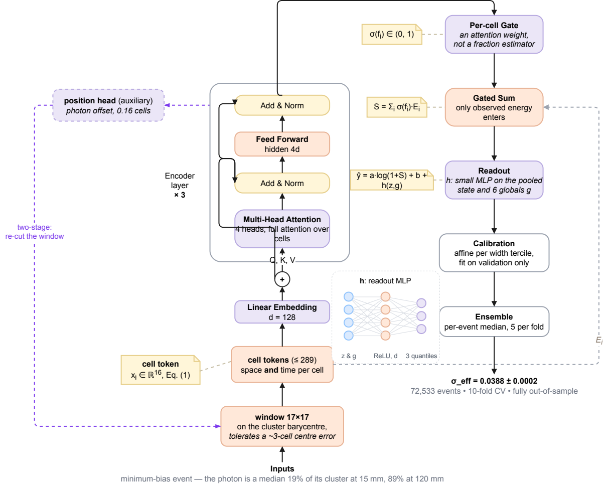
Figure 2: The SpaceFormer pipeline. Each cell is a token in detector space and time; the encoder is a plain transformer over cell tokens only; the cluster-level global features g enter only at the readout, which is a gated energy sum in log space plus a small correction h ; the loss is a three-quantile pinball loss with EMA weights; predictions are the per-event median over ensemble members; the inset draws h itself, a one-hidden-layer network from the pooled state and the globals to the three quantiles. The decisive components are the window’s size and centring at the bottom (Section 5.2). Dashed purple: the auxiliary position head and the two-stage path that re-cuts the window around the predicted photon position (Section 5.3).
