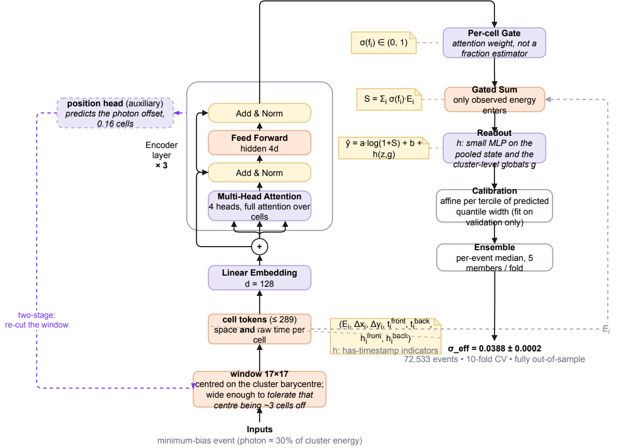
Figure 2: The SpaceFormer pipeline. Each cell is a token in detector space and time; the encoder is a plain transformer over cell tokens only; the cluster-level global features g enter only at the readout, which is a gated energy sum in log space plus a small correction h ; the loss is a three-quantile pinball loss with EMA weights; predictions are the per-event median over ensemble members. The decisive components are the window's size and centring at the bottom (Section 5.2). Dashed purple: the auxiliary position head and the two-stage path that re-cuts the window around the predicted photon position (Section 5.3).
