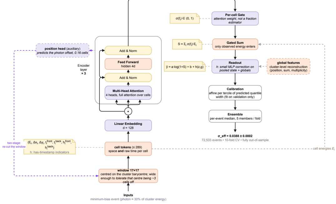
Figure 2: The SpaceFormer pipeline. Each cell is a token in detector space and time; the encoder is a plain transformer over cell tokens only; the cluster-level global features enter at the readout, which is a gated energy sum in log space plus a small correction; the loss is a three-quantile pinball loss with EMA weights; predictions are the per-event median over ensemble members. The decisive components are the window’s size and centring at the bottom (Section 5.2). Dashed purple: the auxiliary position head and the two-stage path that re-cuts the window around the predicted photon position (Section 5.3).
