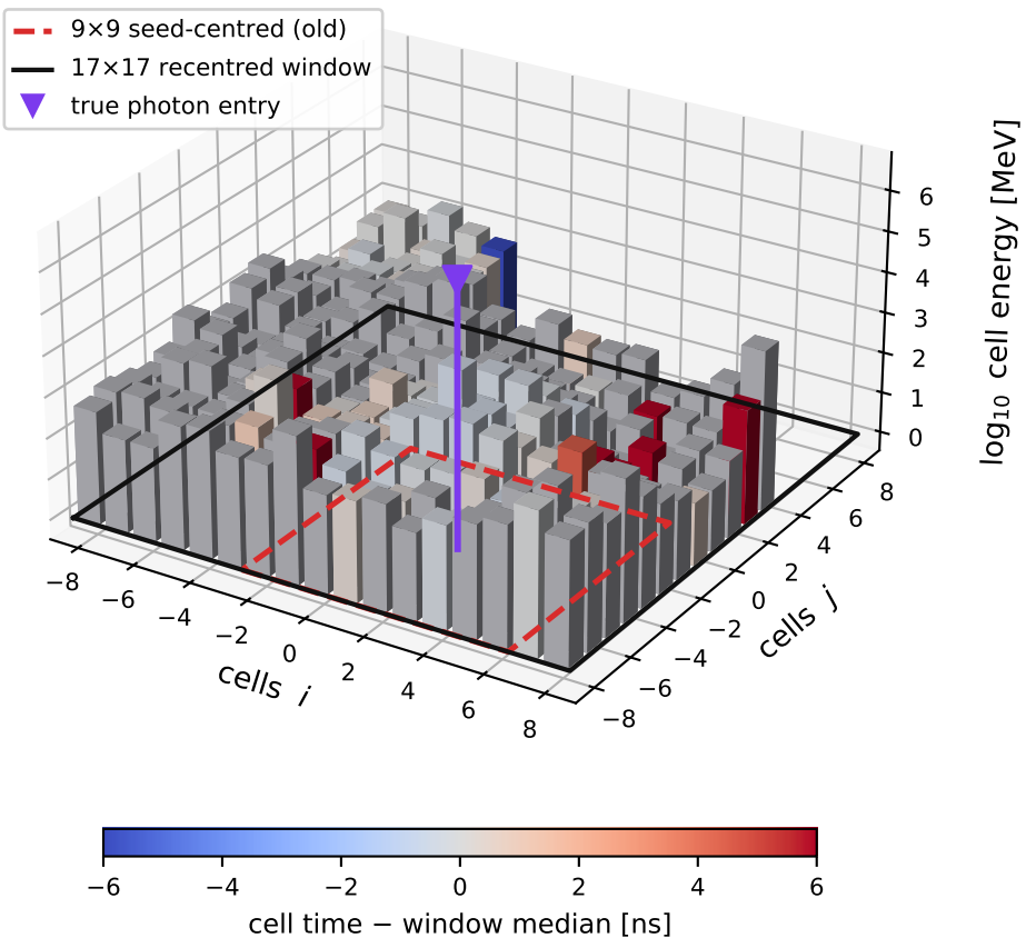
(a) one cluster as space--time tokens
