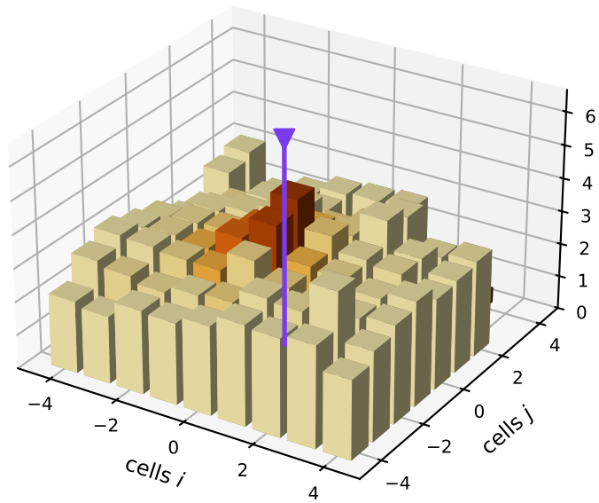
(a) what the detector reads 100% of the window energy
