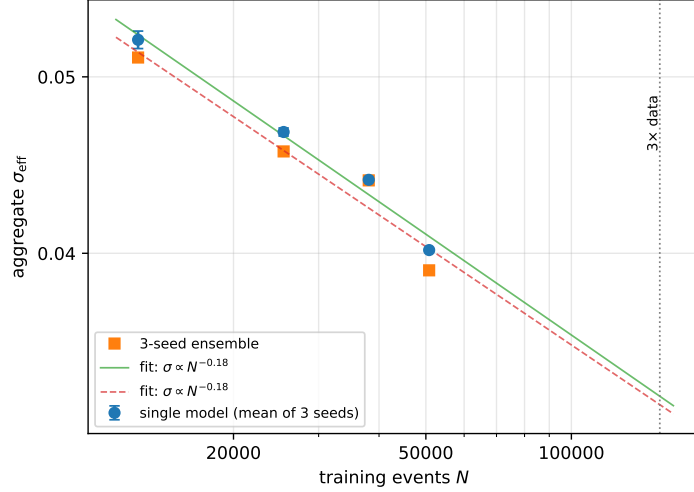
Figure 15: The measured data-scaling curve: aggregate \sigma_{\text{eff}} of the final configuration retrained on 25/50/75/100% of the training set (fixed-split protocol, three seeds per point; the 75% point completed one seed). Both the single-model mean and the three-seed ensemble fit \sigma_{\text{eff}} \propto N^{-0.18} ; the dotted line marks a tripled sample, at a predicted aggregate of \approx 0.033 .
