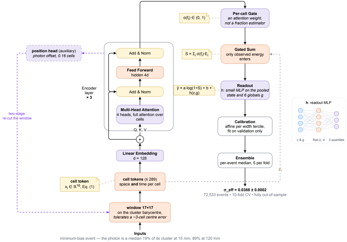
Figure 2: The SpaceFormer pipeline. Each cell is a token in detector space and time; the encoder is a plain transformer over cell tokens only; the cluster-level global features g enter only at the readout, which is a gated energy sum in log space plus a small correction h ; the loss is a three-quantile pinball loss with EMA weights; predictions are the per-event median over ensemble members; the inset draws h itself, a one-hidden-layer network from the pooled state and the globals to the three quantiles. The decisive components are the window’s size and centring at the bottom (Section 5.2). Dashed purple: the auxiliary position head and the two-stage path that re-cuts the window around the predicted photon position (Section 5.3).
