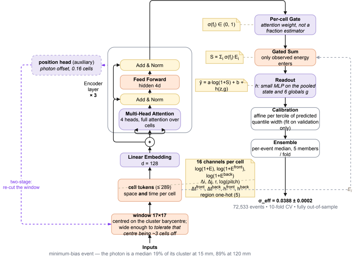
Figure 2: The SpaceTformer pipeline. Each cell is a token in detector space and time; the encoder is a plain transformer over cell tokens only; the cluster-level global features g enter only at the readout, which is a gated energy sum in log space plus a small correction h ; the loss is a three-quantile pinball loss with EMA weights; predictions are the per-event median over ensemble members. The decisive components are the window’s size and centring at the bottom (Section 5.2). Dashed purple: the auxiliary position head and the two-stage path that re-cuts the window around the predicted photon position (Section 5.3).
