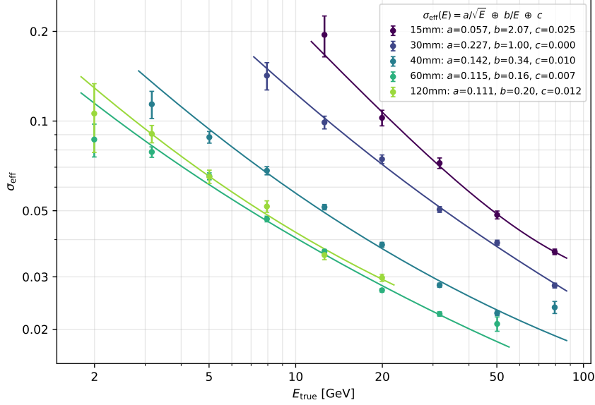
Figure 5: \sigma_{\text{eff}} versus true energy per region (cross-validated ensemble, bootstrap errors) with the standard parameterisation \sigma_{\text{eff}}(E) = a/\sqrt{E} \oplus b/E \oplus c fitted per region. The b (noise) term absorbs the energy-independent pileup contamination and is an order of magnitude larger in the 15 mm region than in the outer ones.
