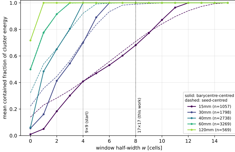
Figure 8: Mean contained fraction of cluster energy versus window half-width w , per region, on the minimum-bias sample (12 files, 9,431 events), for barycentre-centred (solid) and seed-centred (dashed) windows. The vertical lines mark the starting 9 \times 9 window and this work’s 17 \times 17 . At w=4 the 15 mm region is the only one below half containment.
