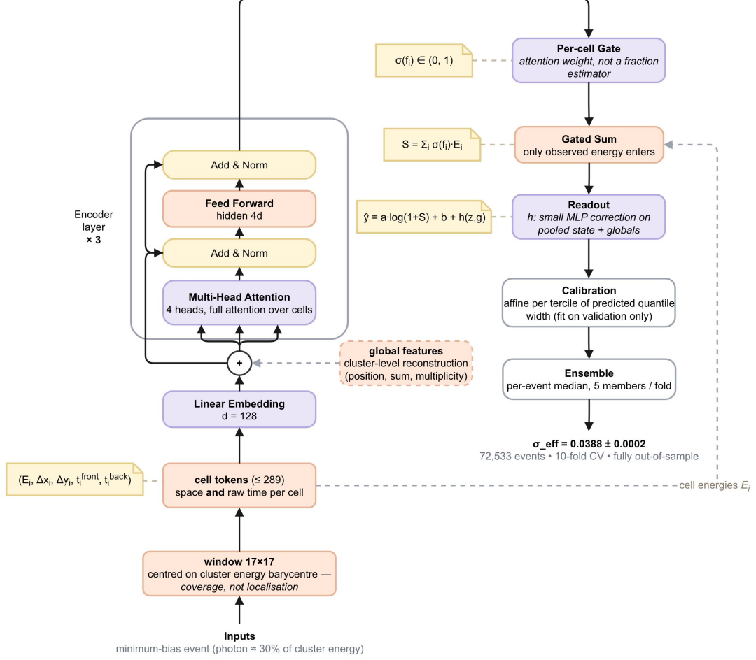
Figure 1: The SpaceFormer pipeline. Each cell is a token in detector space and time; the encoder is a plain transformer; the readout is a gated energy sum in log space; the loss is a three-quantile pinball loss with EMA weights; predictions are the per-event median over ensemble members. The two decisive components are on the far left: window size and window centring (Section 5.2).
