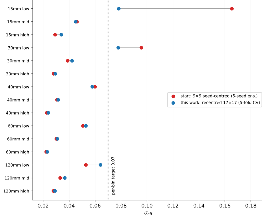
Figure 3: All fifteen region–energy bins: starting configuration (red, fixed-split five-seed ensemble) versus this work (blue, cross-validated ensemble). The two protocols differ slightly (Section 3); the dominant moves — 15 mm low 0.165 \rightarrow 0.078 , 30 mm low 0.096 \rightarrow 0.078 — dwarf that difference.
