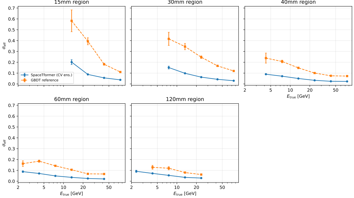
Figure 4: \sigma_{\text{eff}} versus true photon energy per region: SpaceTformer (cross-validated ensemble, circles) against the six-feature GBDT reference (single model, fixed split, squares). Error bars are bootstrap errors over test events. The gain is largest at low energy and in the inner regions, matching the pileup-contamination pattern.
